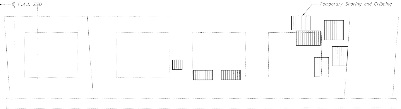
ELEVATION - PIER F, NORTH FACE
