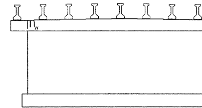
PIER 2 ELEVATION, SOUTH FACE (LOOKING NORTH)
