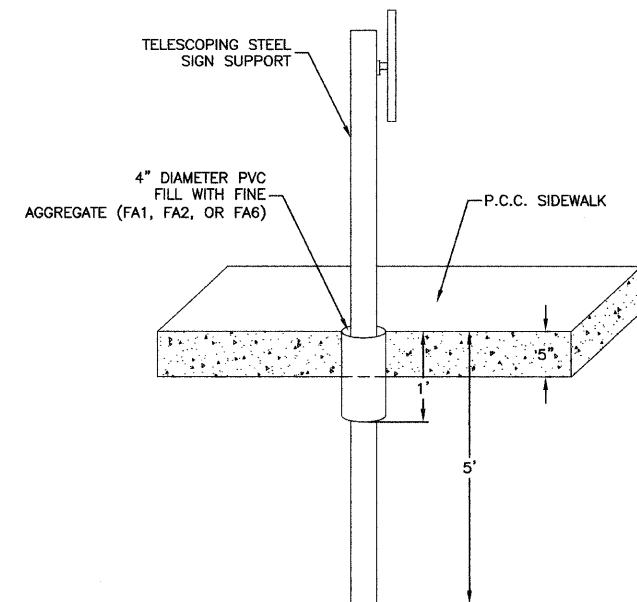
SIGN SUPPORT MOUNTING DETAIL
