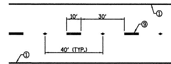
TYPICAL PAVEMENT MARKING (STA. 507+00 TO STA. 34+04)
