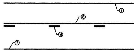
TYPICAL PAVEMENT MARKING - NO PASS ZONE (SEE SCHEDULE FOR LOCATIONS)
