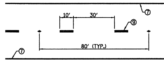
TYPICAL PAVEMENT MARKING (STA. 373+85 TO STA. 507+00)
