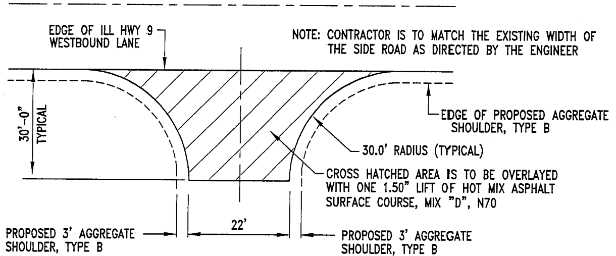
TYPICAL PLAN VIEW OF INTERSECTION AT ILL HWY 9
