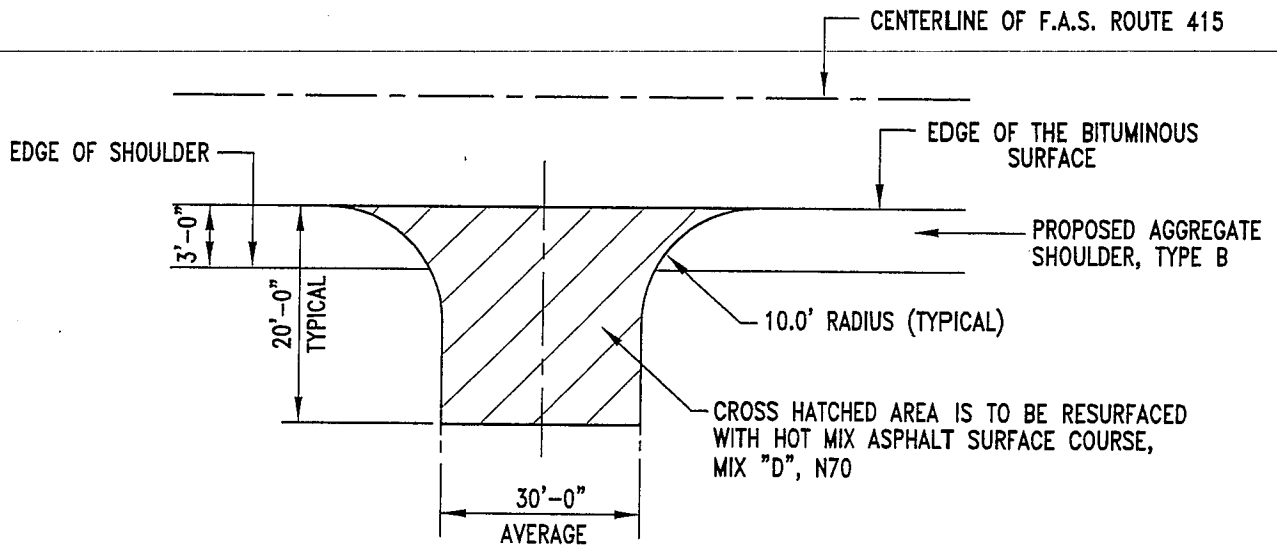
TYPICAL DETAIL OF 3 SCHOOL ENTRANCES
