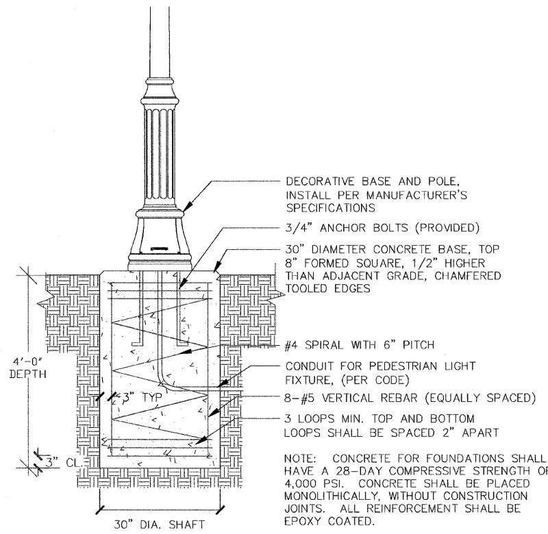
L 2-2 LIGHTS, PEDESTRIAN & DECORATIVE SIGN BASE NOT TO SCALE
