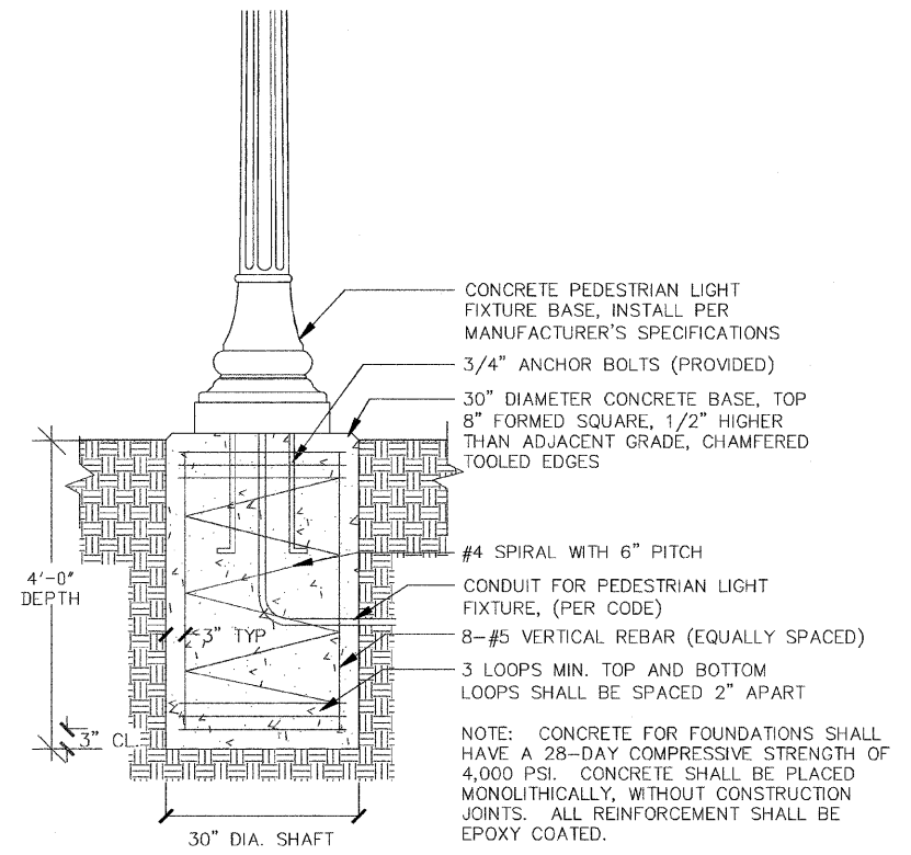
L 2-3 LIGHTS, GLOBE ON CONCRETE POLE NOT TO SCALE
