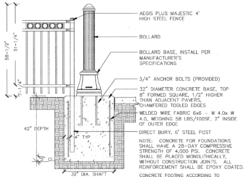
L 2-4 BOLLARD BASE AND FENCE POST (1) NOT TO SCALE
