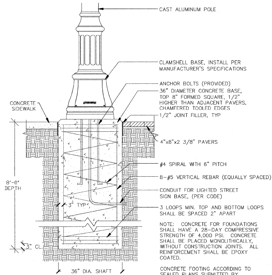
L 2-1 LIGHTS, STREET NOT TO SCALE
