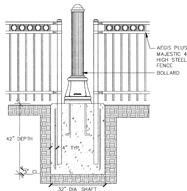
L 2-5 BOLLARD AND FENCE POSTS (2) NOT TO SCALE
