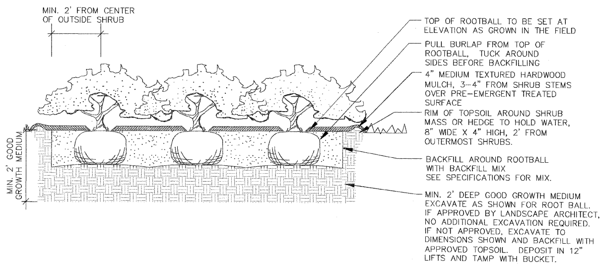
L 4-3 SHRUB BEDS AND HEDGES NOT TO SCALE
