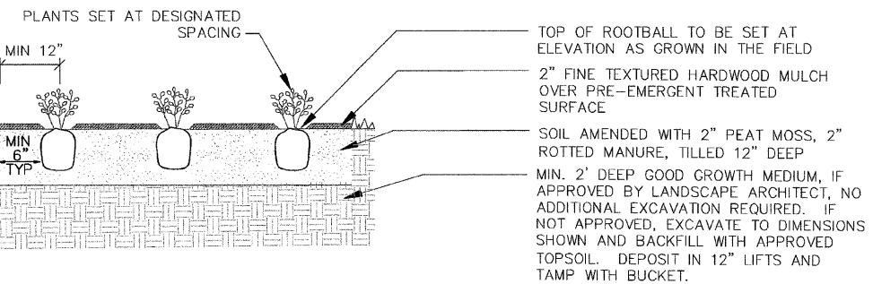
L 4-4 FLOWER AND GROUND COVER BEDS NOT TO SCALE
