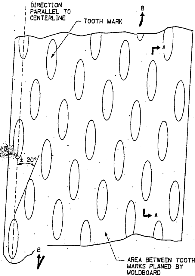
PLAN
