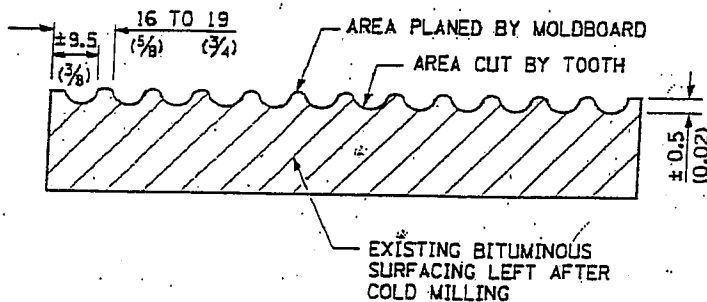
SECTION B-B PROJECTED PERPENDICULAR TO CENTERLINE
