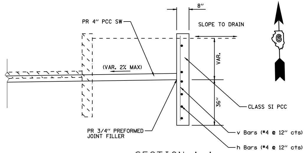
SECTION A-A (PR RETAINING WALL)
