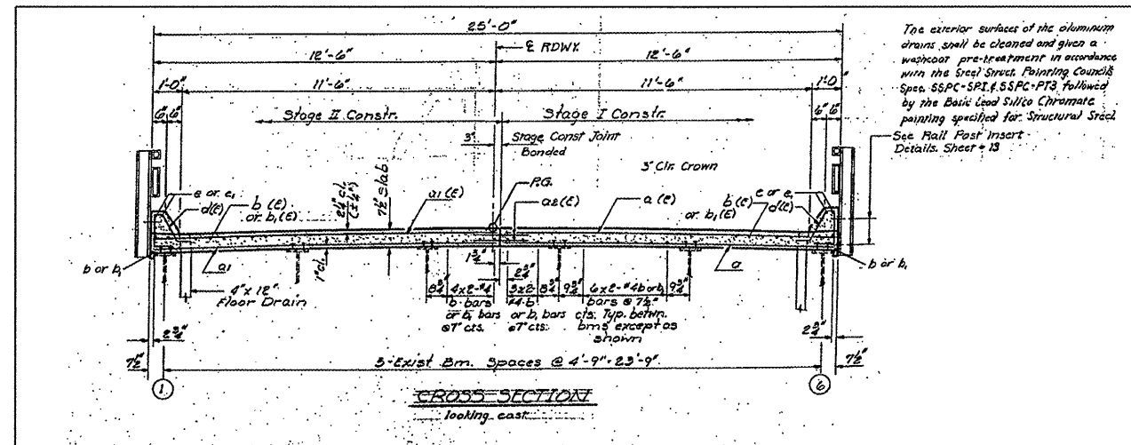
EXISTING SLAB DETAILS - APPROACH SPANS
