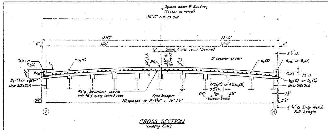
EXISTING SLAB DETAILS - TRUSS SPANS
