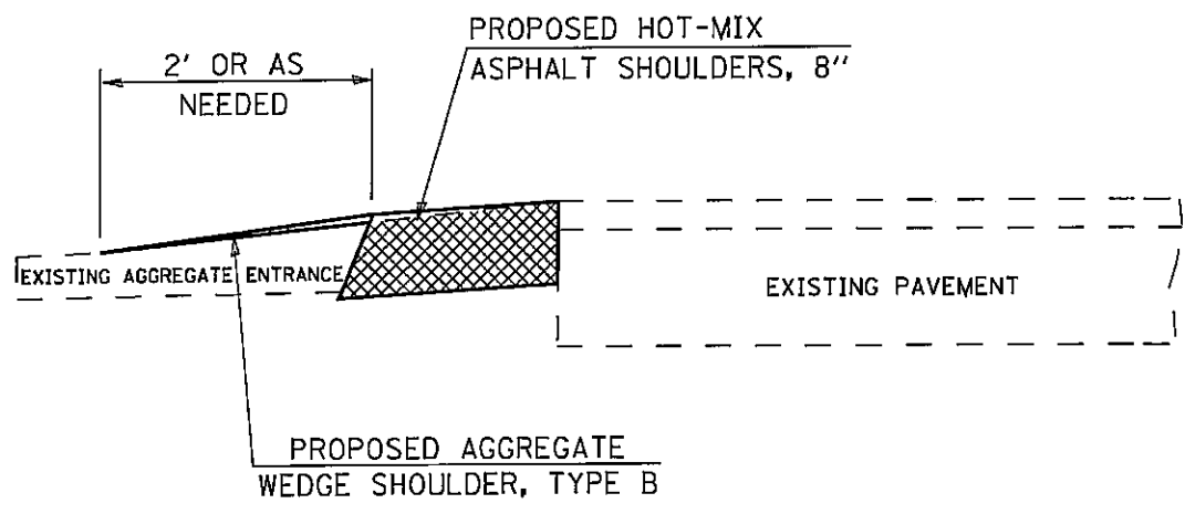
SHOULDER DETAIL AT AGGREGATE ENTRANCES (OMIT SHOULDER RUMBLE STRIP THROUGH WIDTH OF ENTRANCE)
