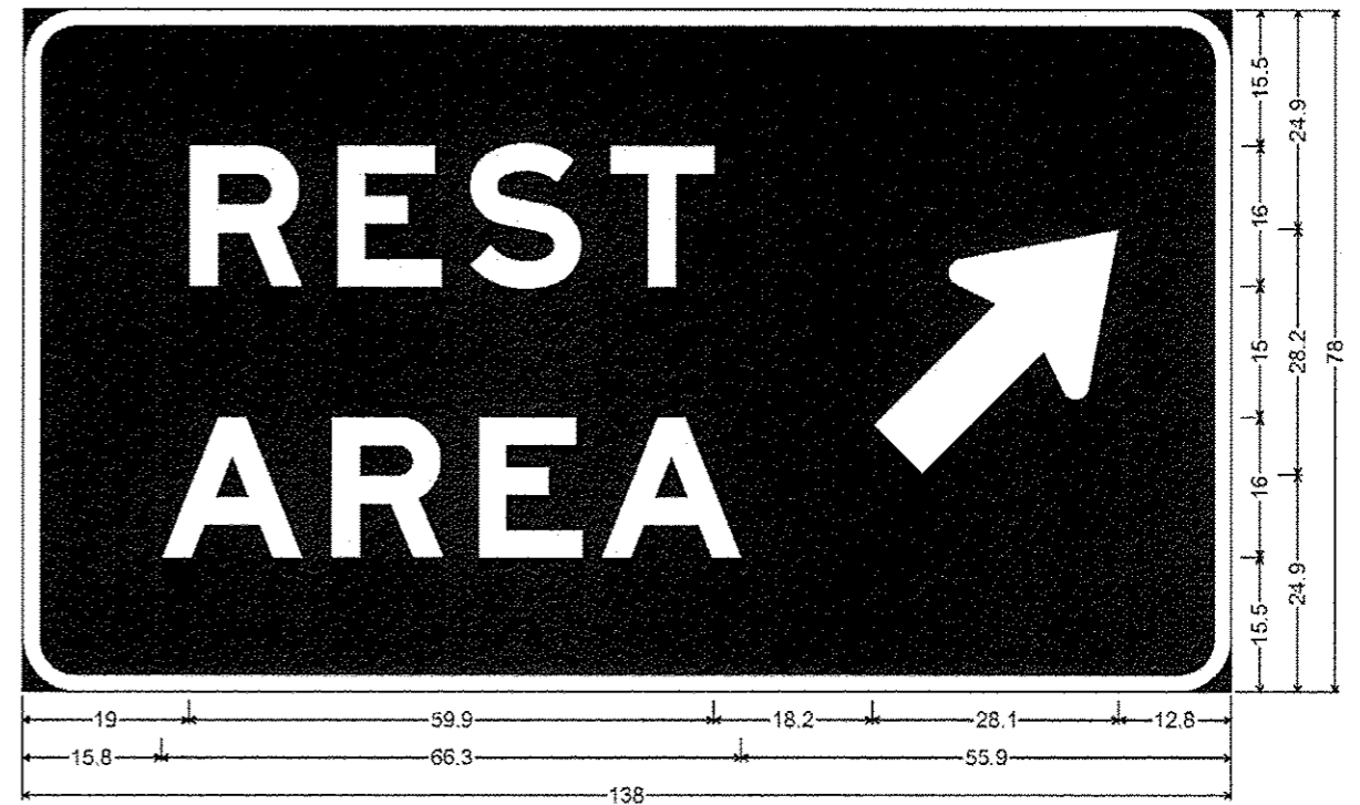
6.0" Radius, 2.0" Border, White on Blue; "REST" E Mod; "AREA" E Mod; Standard Arrow Custom 35.8" X 21.6" 45";
