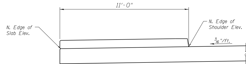
SECTION B-B THRU NORTH SIDEWALK
