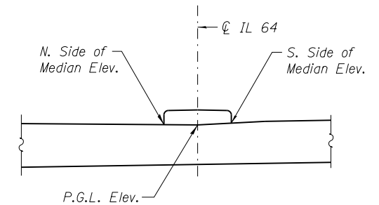
SECTION THRU MEDIAN
