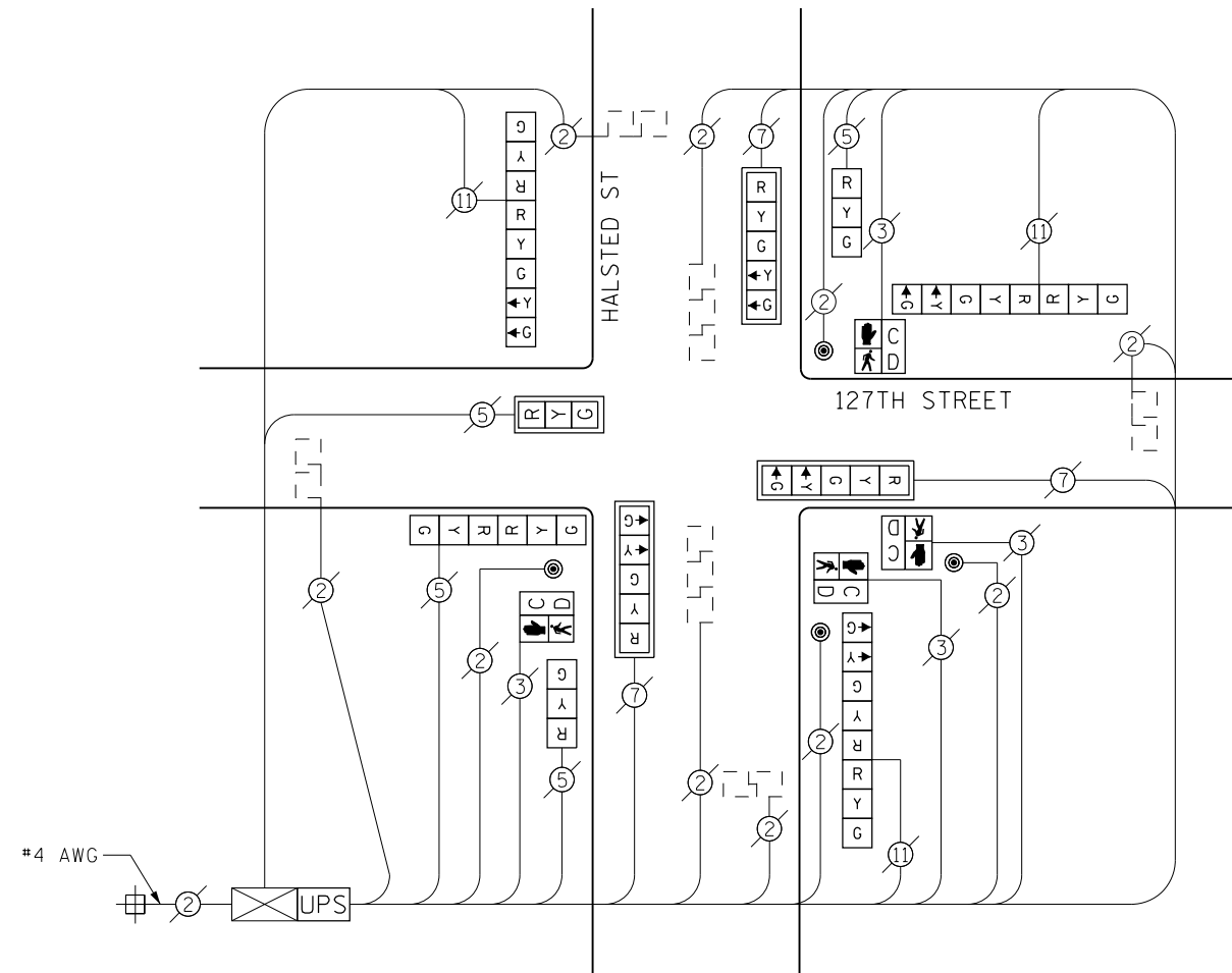
CABLE PLAN
