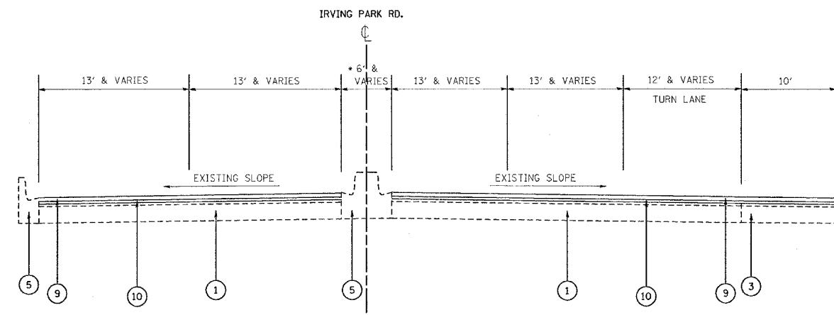
PROPOSED TYPICAL CROSS SECTION
