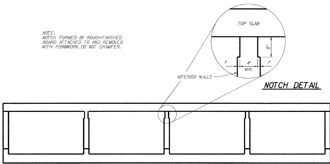
SECTION THRU BARREL NEAR DOWNSTREAM END ONLY
