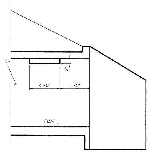
LONGITUDINAL SECTION PHOEBE NESTING SITE DETAILS
