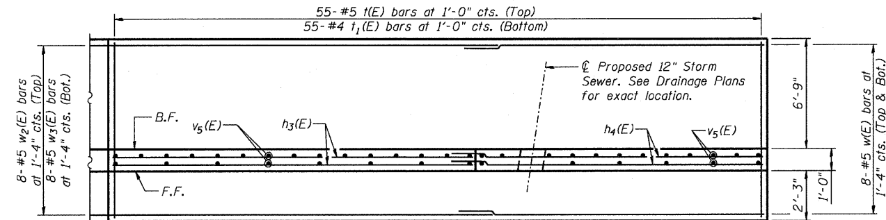
FOOTING PLAN OF PANELS J & K
