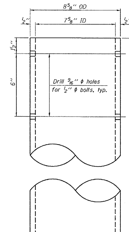
DOWNSPOUT
