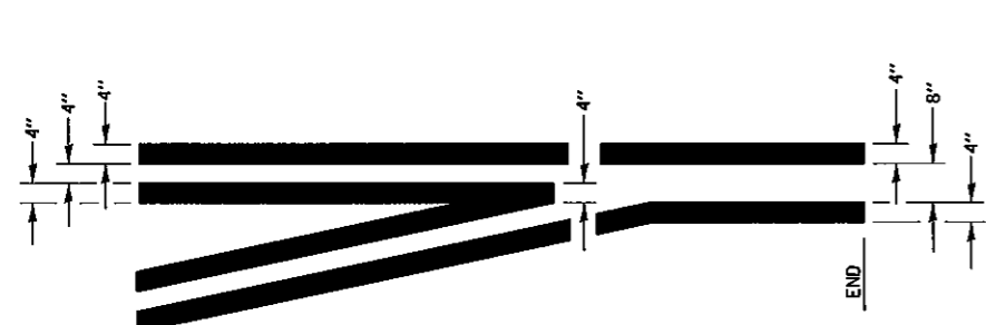
TYPICAL APPLICATION @ LEFT TURN LANES
