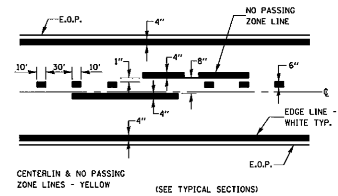
PAVEMENT MARKING
