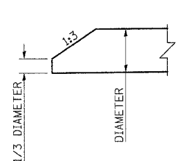
SECTION VIEW OF MITERED END MITERED ENDS TO BE INCLUDED IN THE TOTAL LENGTH OF THE PIPE
