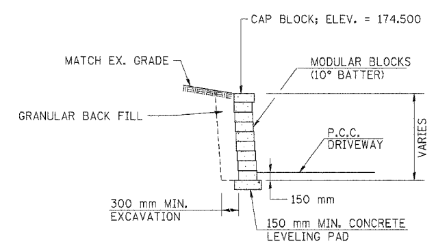
MODULAR RETAINING WALL SYSTEM
