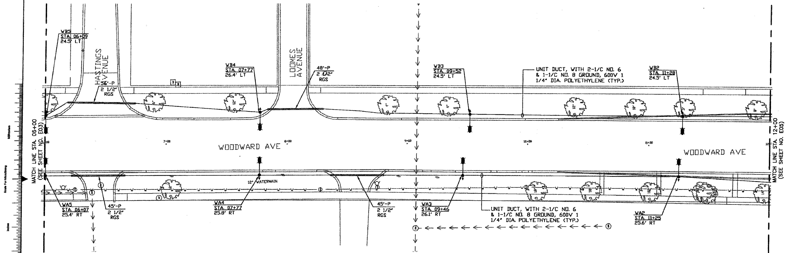
PARTIAL WOODWARD AVENUE LIGHTING LAYOUT - PROPOSED PLAN SCALE AS NOTED
