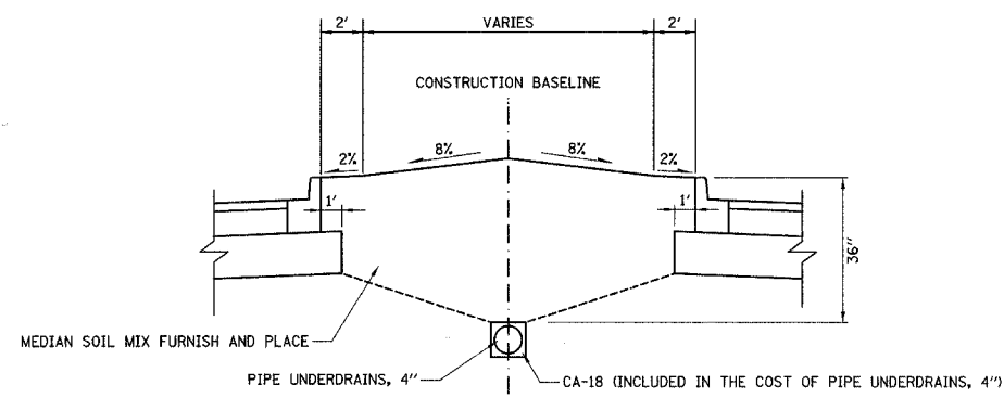
LANDSCAPE MEDIAN DETAIL NOT TO SCALE
