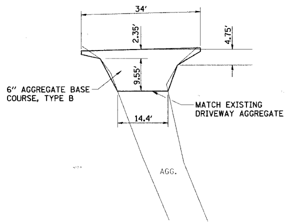
PRIVATE ENTRANCE DETAIL STA. 16+82.83
