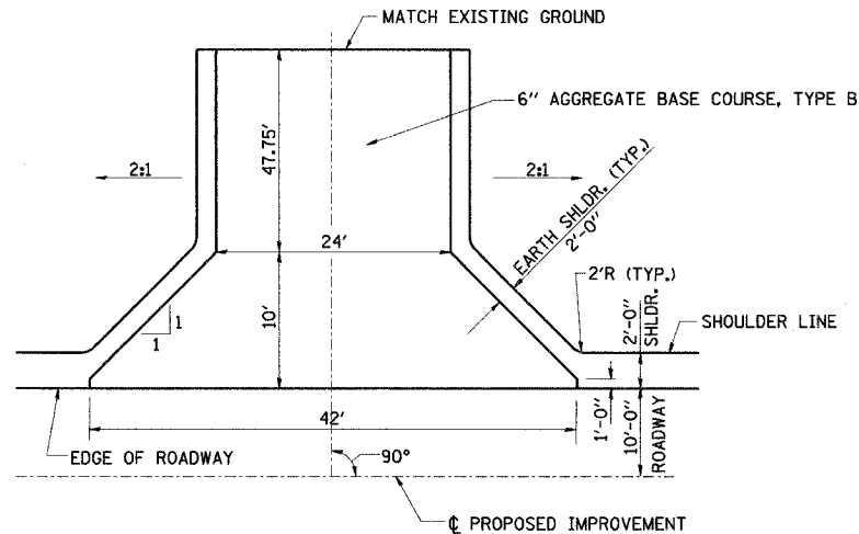
FIELD ENTRANCE DETAIL STA. 13+50.00
