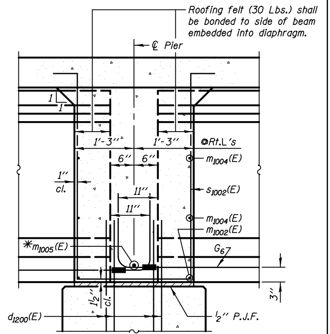
SECTION B-B
