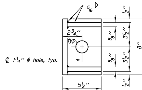
SIDE RETAINER
