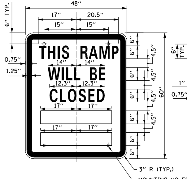
SIGN TS-4
