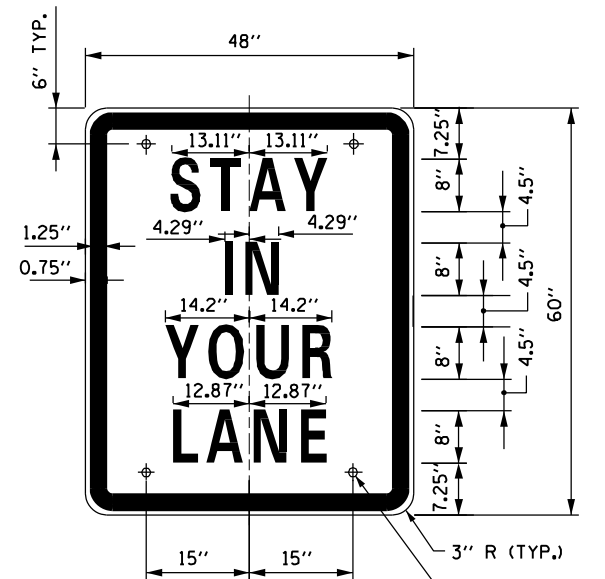
SIGN TS-3
