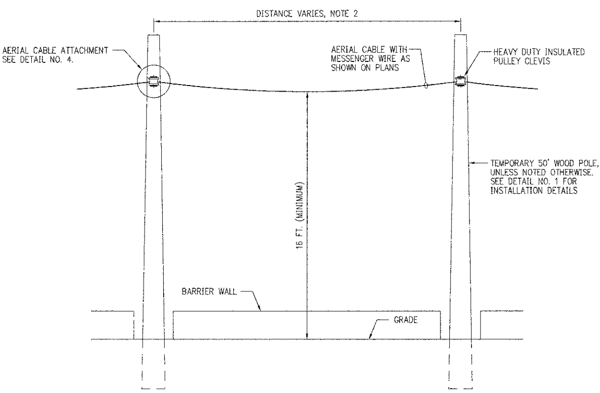
3 AERIAL CABLE INSTALLATION DETAIL NOT TO SCALE
