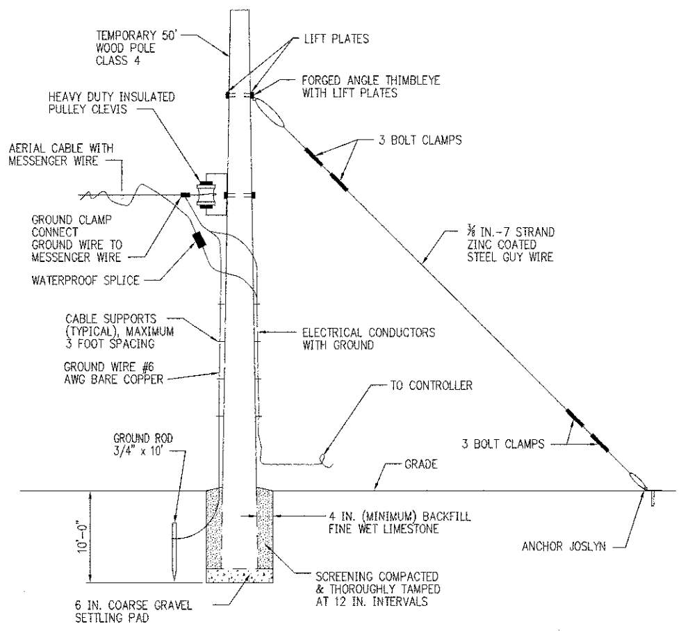
2 TEMPORARY WOOD END POLE INSTALLATION DETAILS NOT TO SCALE
