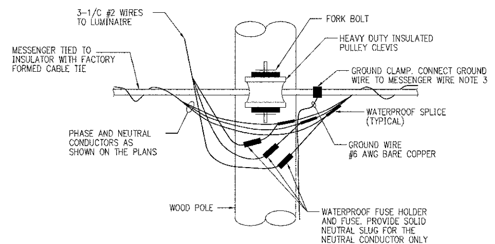
4 TEMPORARY WOOD POLE AERIAL CABLE ATTACHMENT DETAIL NOT TO SCALE
