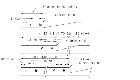
TYPICAL PAINTED MEDIAN MARKING
