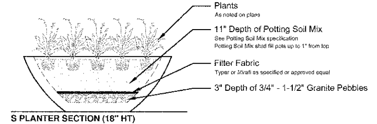
S PLANTER SECTION (18" HT)
