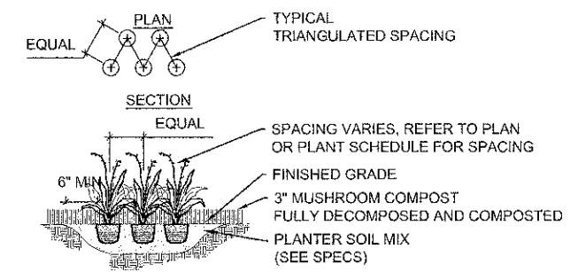
3 GROUNDCOVER / PERENNIALS SCALE= 3/4"=1'-0"
