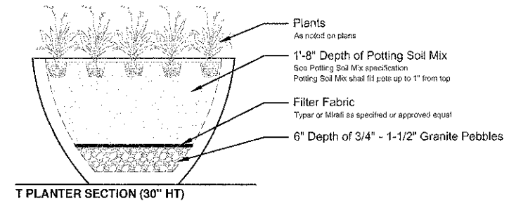
T PLANTER SECTION (30" HT)
