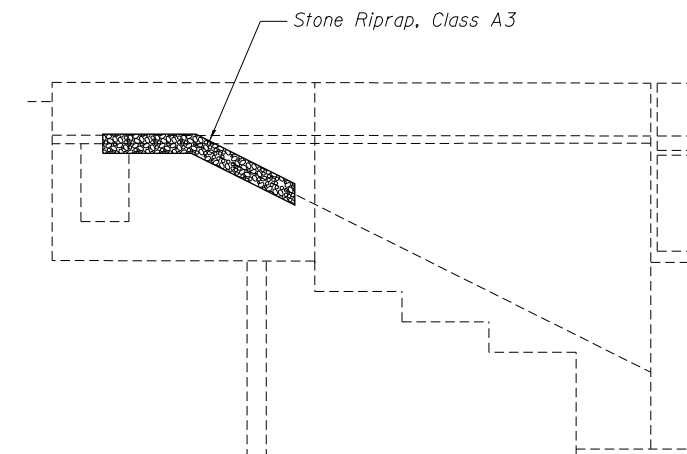
RIPRAP PLACEMENT ON SLOPE
