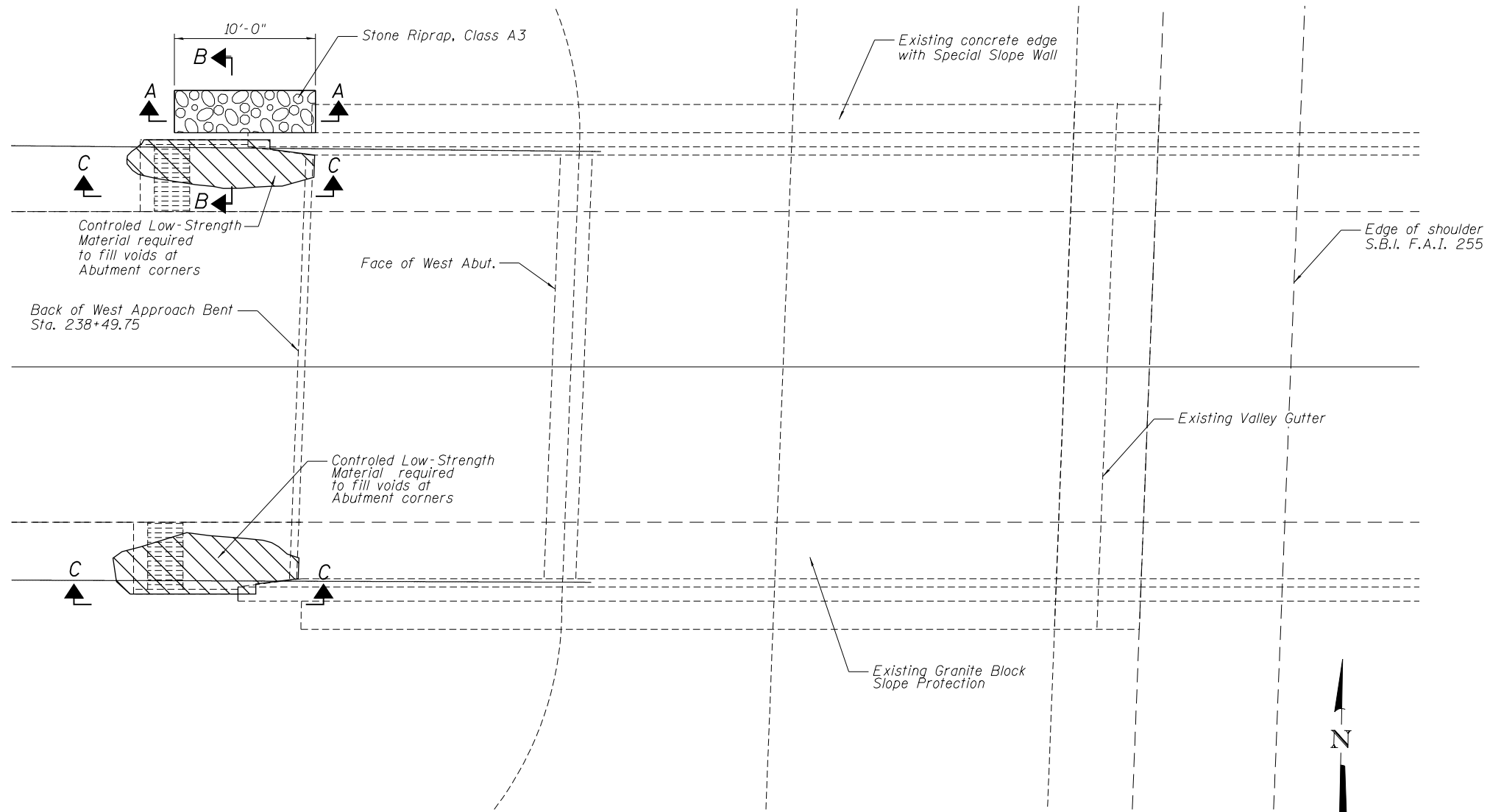
WEST SLOPEWALL PLAN
