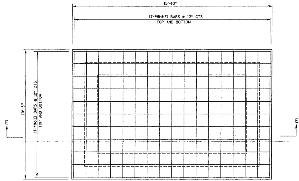
PLAN BOTTOM SLAB
