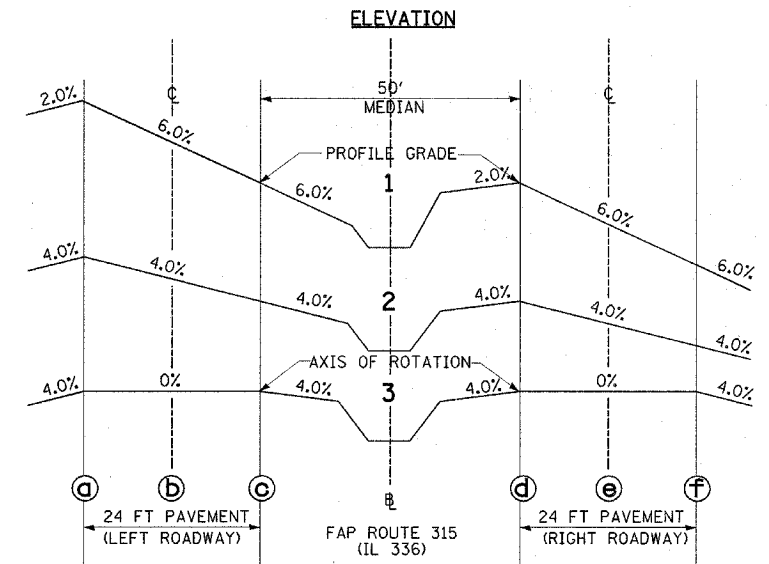
CROSS SECTIONS
