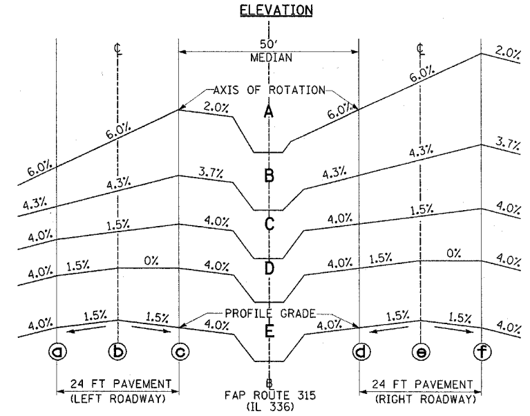
SUPERELEVATION DETAILS (SE REMOVED STA 13+45.52 TO 16+54.52)
