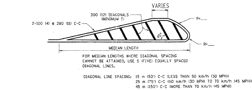
MEDIANS OVER 1.2 m (4') WIDE
