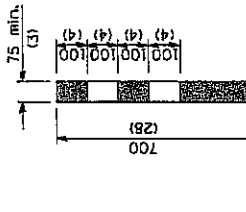
FLEXIBLE DELINEATOR
