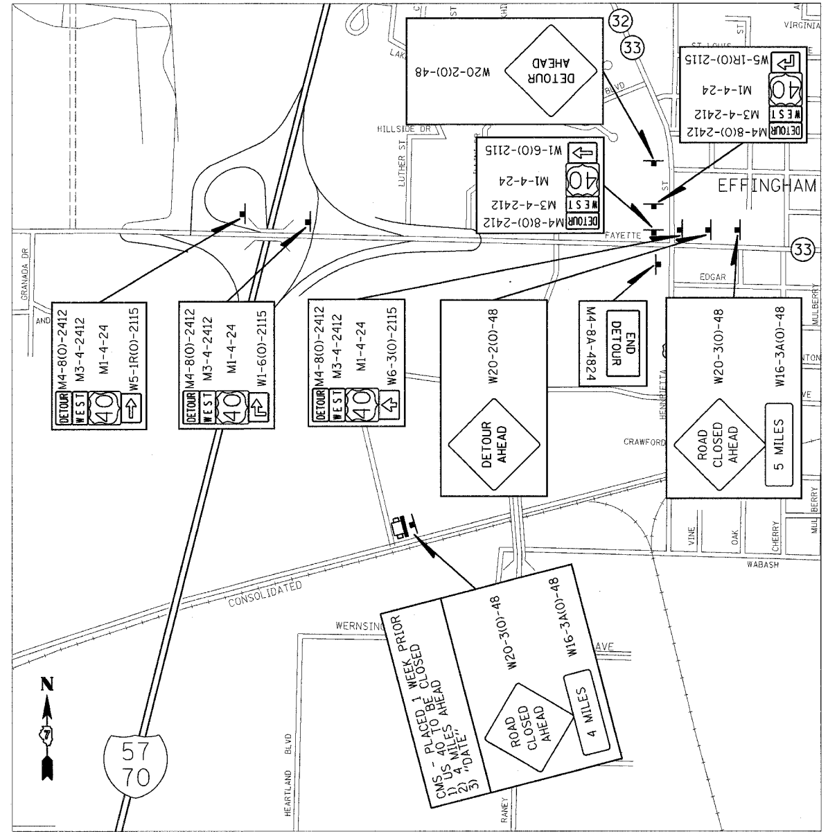
DETOUR DETAIL 2
