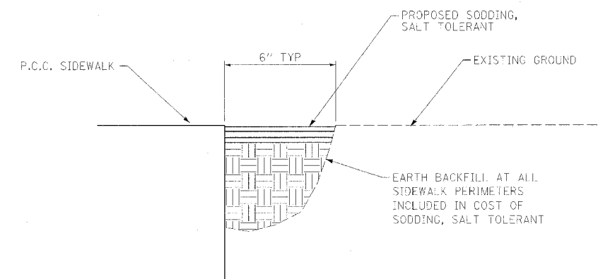
EARTH BACKFILL AT SIDEWALKS
