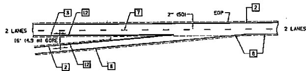
TYPICAL ENTRANCE RAMP TERMINAL
