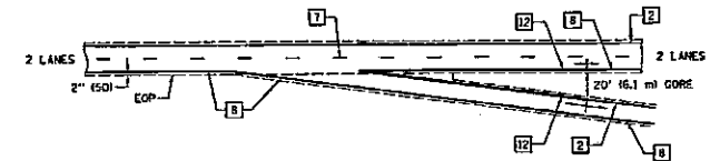
TYPICAL PAVEMENT MARKING LEGEND
