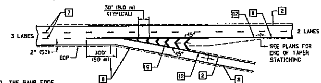
EXIT RAMP TERMINAL with EXCLUSIVE (auxiliary) LANE
