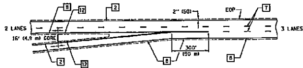
ENTRANCE RAMP TERMINAL with EXCLUSIVE LANE
