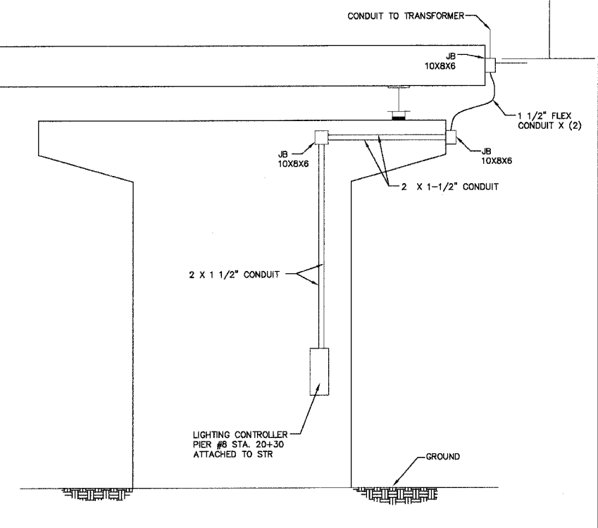
LIGHTING CONTROLLER AND CONDUIT LAYOUT @ STA. 20+30
