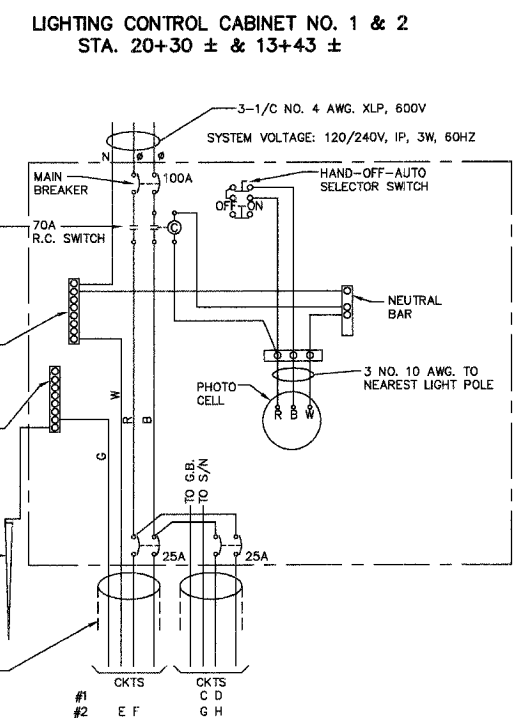
LIGHTING CONTROL CABINET SOUTH ABUTMENT STA. 13+43 ± #1 PIER #8 STA. 20+30 ± #2
