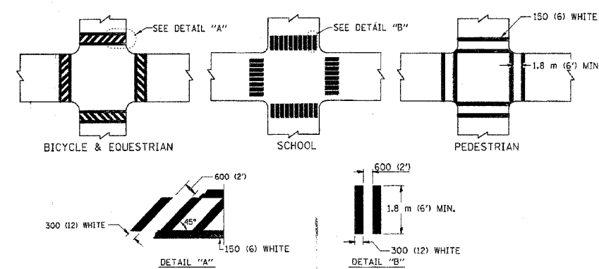
TYPICAL CROSSWALK MARKING \\GLENDALEHEIGHTS\0451C22\01\0451C22.std.pin
