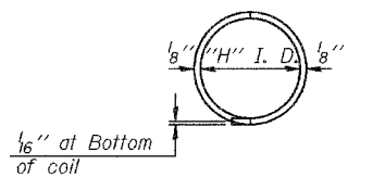
PLAN-COIL WIRE
