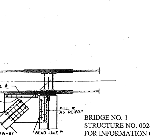
SECTION F22-F22
