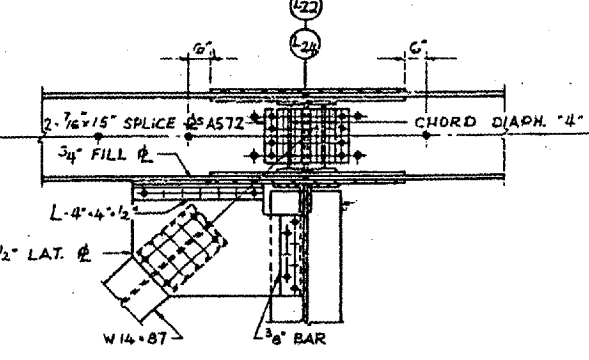
SECTION F20-F20
