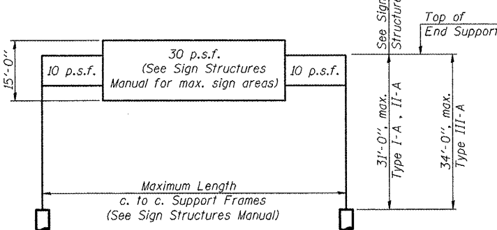
DESIGN WIND LOADING DIAGRAM Parameters shown are basis for I.D.O.T. Standards and Sign Manual Tables. Installations not within dimensional limits shown require special analysis for all components.
