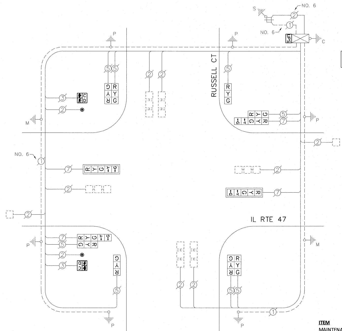
CABLE PLAN
