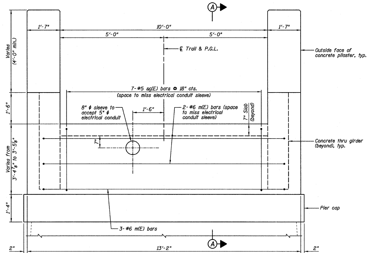
DIAPHRAGM @ PIER NO. 3
