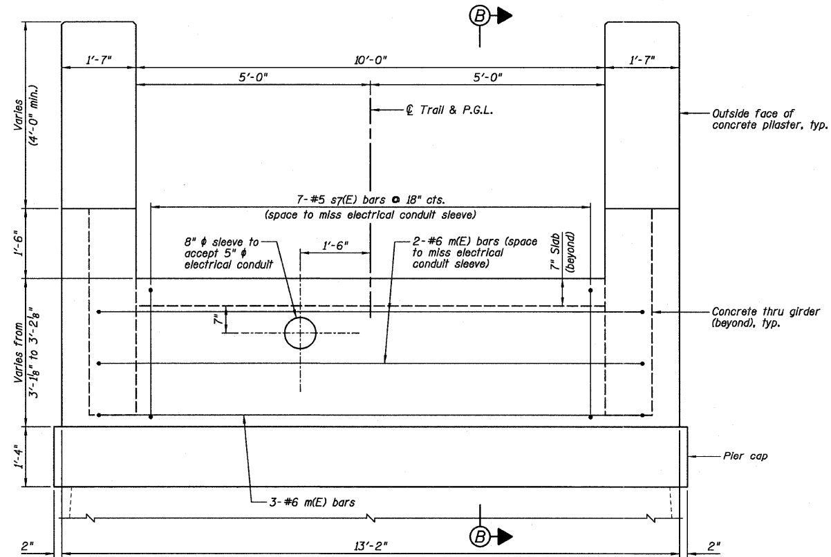
DIAPHRAGM @ PIER NO. 4
