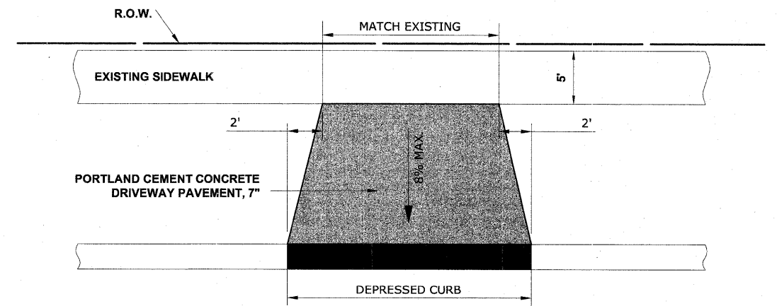
DRIVEWAY DETAIL
