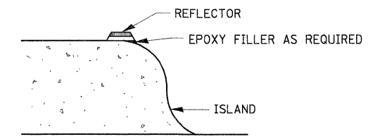
SECTION VIEW
