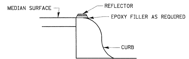
SECTION VIEW
