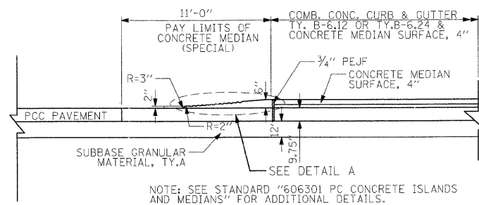
CONCRETE MEDIAN (SPECIAL) DETAIL AT NEEDHAM ROAD INTERSECTION
