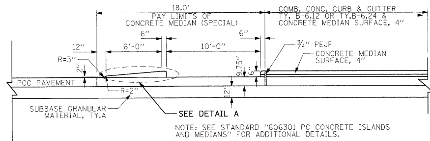
CONCRETE MEDIAN (SPECIAL) DETAIL AT WAUBONSEE DRIVE INTERSECTION
