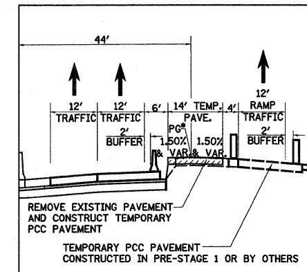
DETAIL D-D
