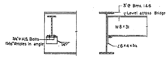
DIAPHRAGM D No. Req'd: 10 Each Unit
